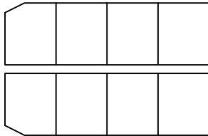
Side Skirts for PzKpfw III Ausf. L/M/N Type D
